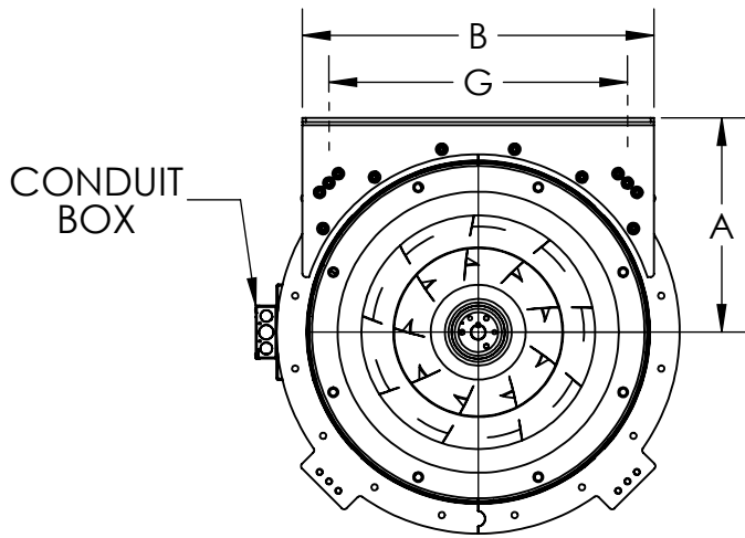
INLET VIEW
